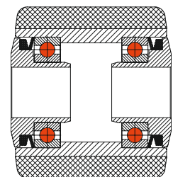
V-ring sealing gasket
