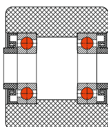
Labyrinth sealing
