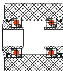
V-ring sealing gasket
