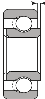
Axial Internal Clearance
